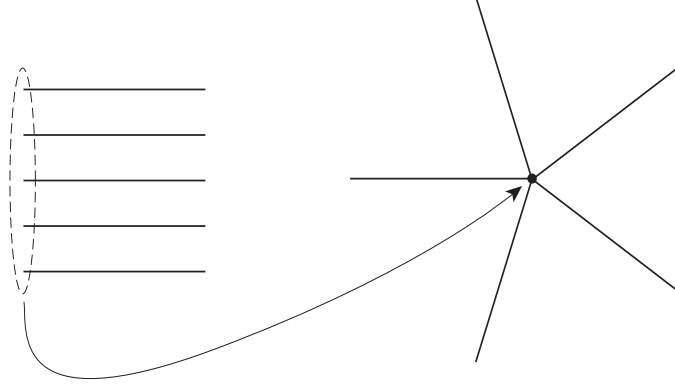
FIGURE 1. Walsh's Spider. Left-hand endpoints are mapped into vertex
