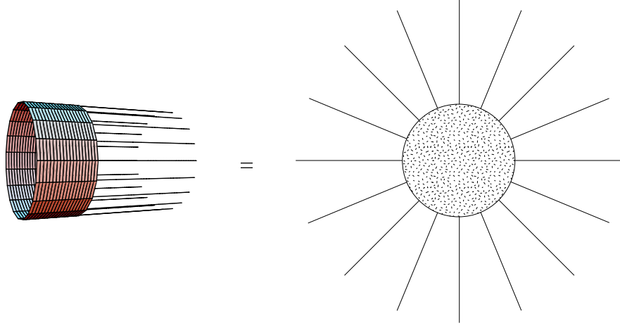
FIGURE 4. The daisy and cylinder.
