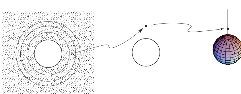
FIGURE 3. Lollipop. Unit ball is mapped into sphere and exterior of unit ball is mapped into line
