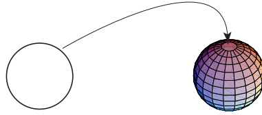
FIGURE 2. Ball to Sphere. Boundary of unit ball is mapped to north pole of sphere
