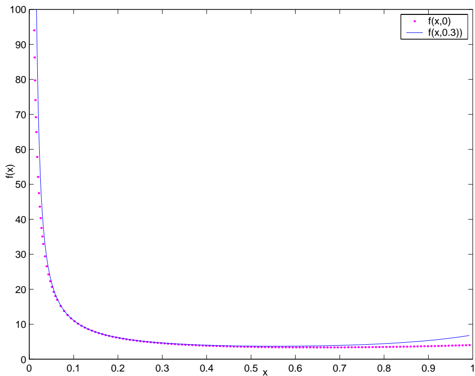
FIGURE 2. Frequency spectrum f(x,t) = g(x,t)/(x(1-x)) at times t = 0 and t = 0.3 with parameter values R = 40 and S = +2 . Obtained by numerically integrating the PDE. The values of f are restricted to the interval [0, 100] .
