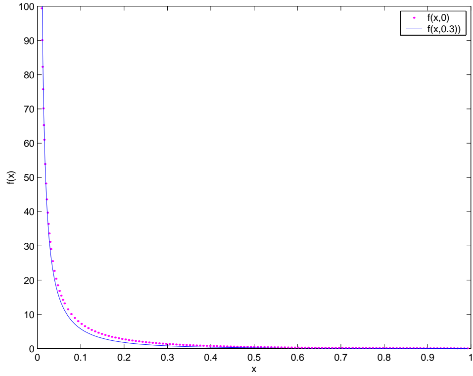
FIGURE 3. Frequency f(x,t) = g(x,t)/(x(1-x)) at times t = 0 and t = 0.3 with parameter values R = 40 and S = -2 ; Obtained by numerically integrating the PDE. The values of f are restricted to the interval [0, 100] .
